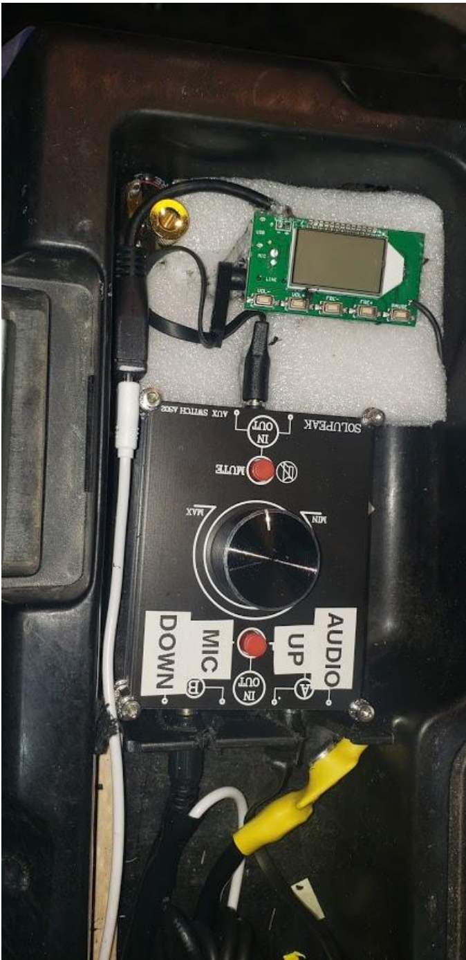
Left Compartment Layout
