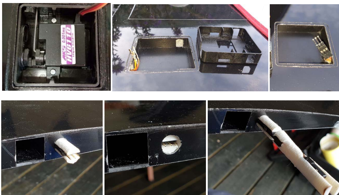
Aileron and flap servo details – below: Contact holder arrangement glued in
