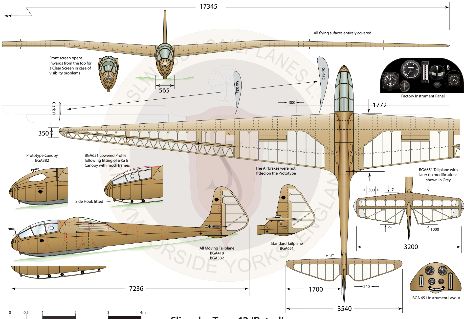
Slingsby Type 13 'Petrel' - 1939
