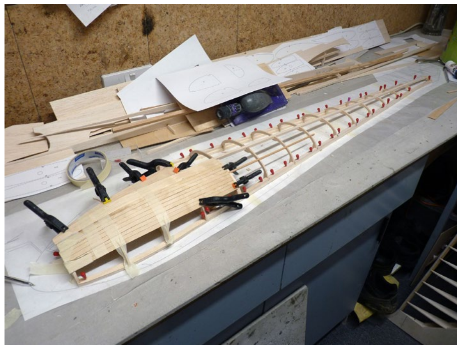
Figure 1. Traditional half-shell fuselage construction.
