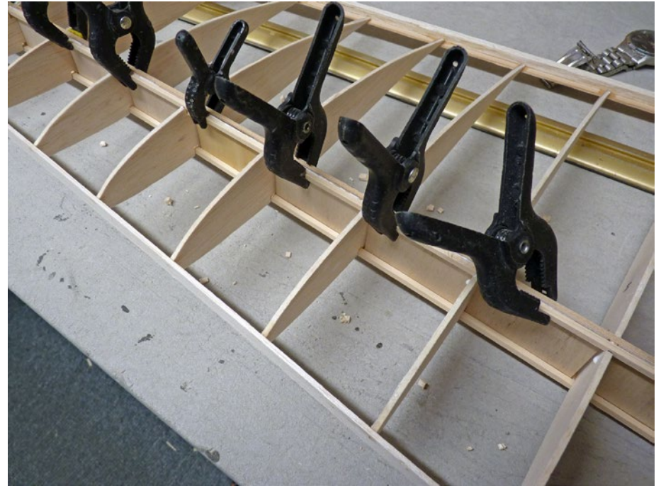
Figure 6. Sub spars added to form H-beam.
